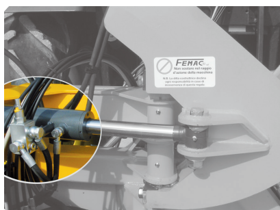
SCHOKBESTENDIGE HYDRAULISCHE BEVEILIGING SHOCK RESISTANT HYDRAULIC SAFETY DEVICE
